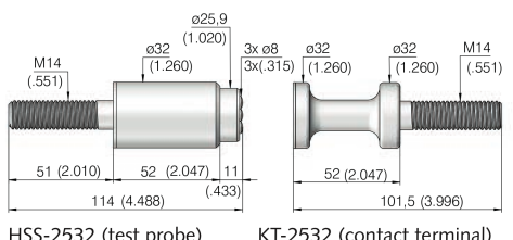
HSS-2532 (test probe) KT-2532 (contact terminal)
