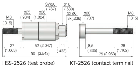
HSS-2526 (test probe) KT-2526 (contact terminal)
