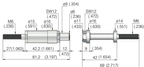
HSS-2516 (test probe) KT-2516 (contact terminal)
