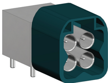
HFM-Male (4-pole)
